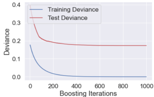
Figure 10. Training and test set deviance
