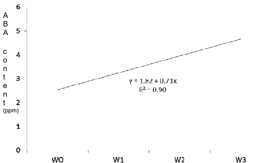
Figure 1. Relationship between Water Stress and ABA Content at Ages 12 WAP
